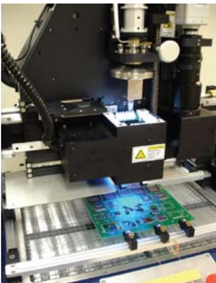
BGA Rework
