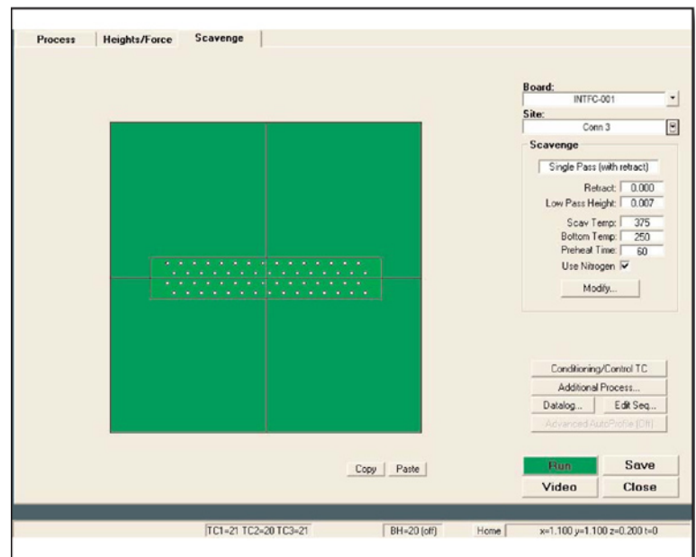
SierraMate™ Scavenger Set-up
